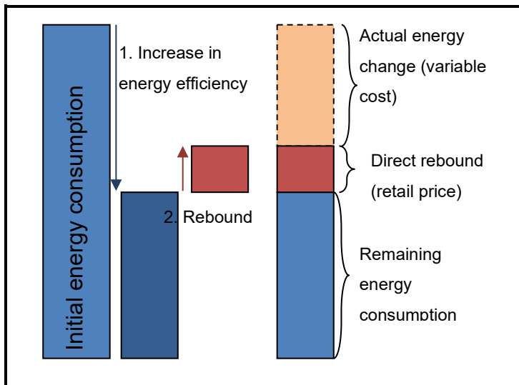
Figure 3.1 Valuing energy changes with direct rebound effects
