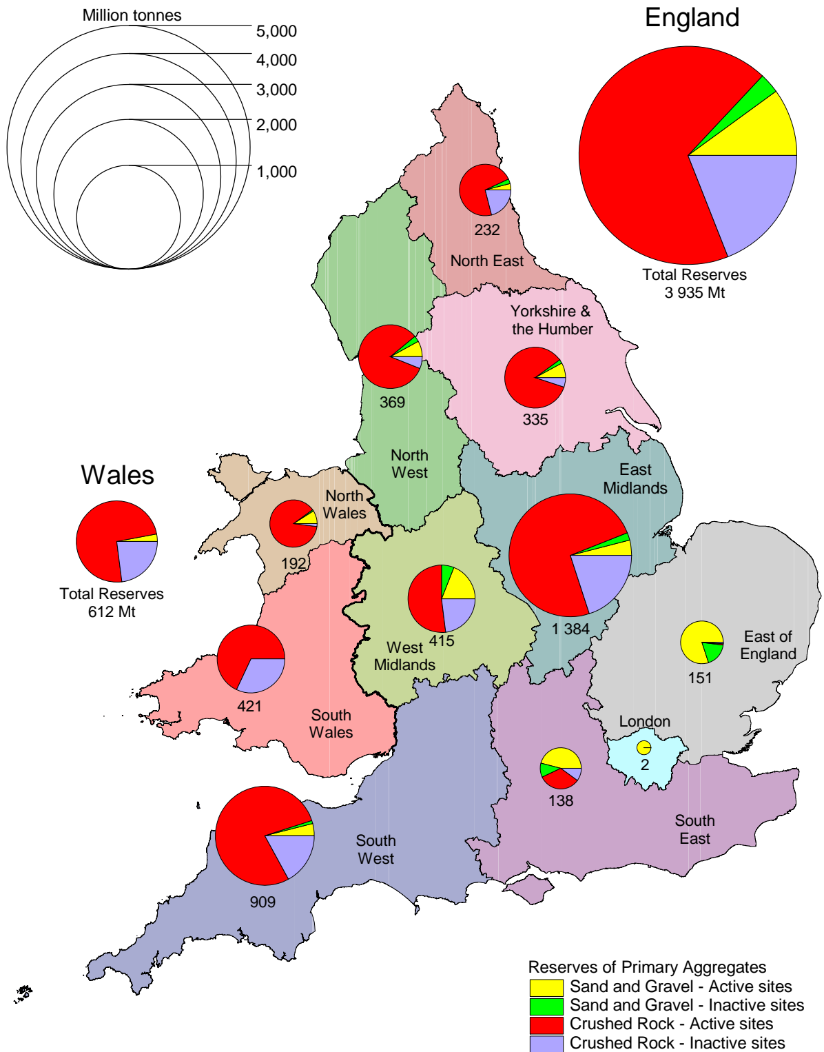
Map 10: Permitted reserves of primary aggregates in England and Wales – active and inactive sites, 2009
