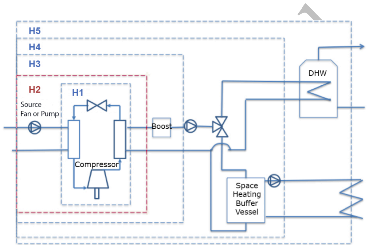
Figure 2-1. SEPEMO system boundaries (derived from Riviere et al., 2011) with the addition of H5 boundary that accounts for heat losses from the hot water cylinder
