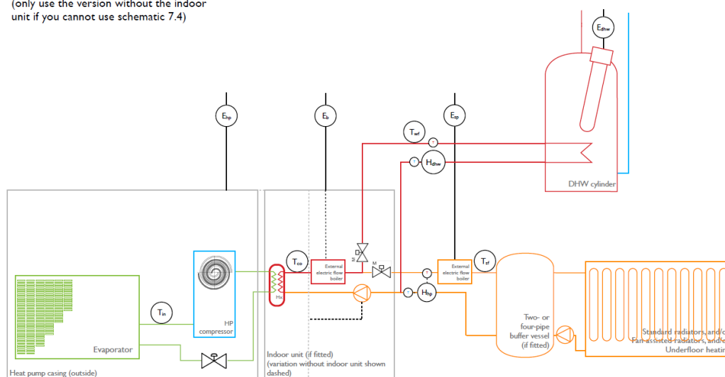
Figure B 1. Schematic of heat pump system with all four possible electricity meters installed.
