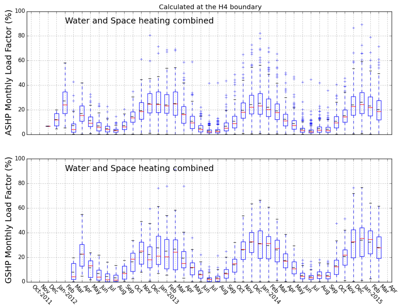
Figure 3-15. Box plots of monthly load factors at H4 system boundary for ASHPs and GSHPs.
