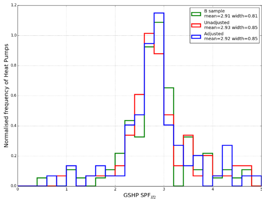
Figure A-8. Histograms of SPF_{H2} for GSHPs in Sample B (green), Sample C unadjusted (red) and Sample C adjusted to UKSET conditions (blue)
