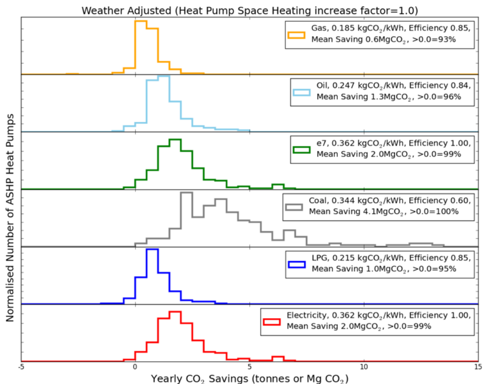
Figure A-12. Histograms of annual CO 2 savings for ASHPs when replacing gas, oil, electricity (E7), Coal, LPG, and Electricity (standard tariff) with data from Sample C adjusted to UKSET
