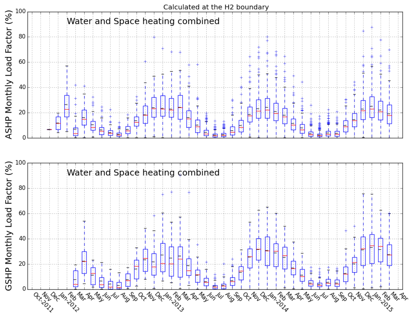
Figure 3-14. Box plots of monthly load factors at H2 system boundary for ASHPs and GSHPs
