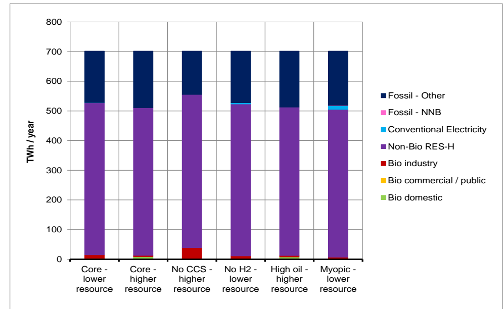
Figure 24 Heat output 2050 (All scenarios)
