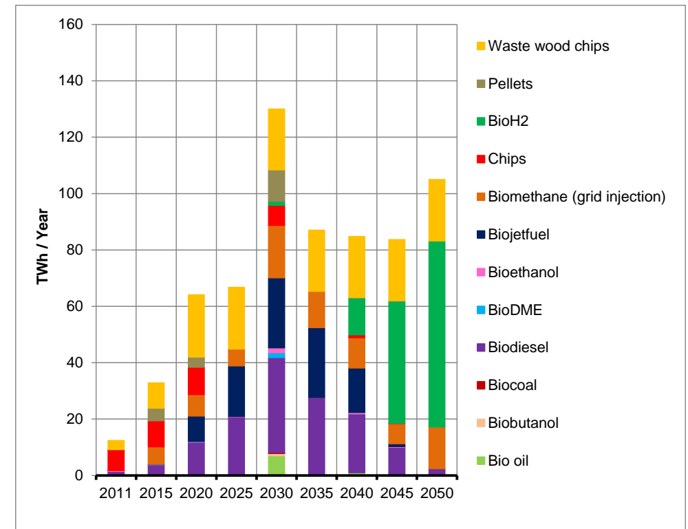
Figure 58 UK bioenergy carrier (Myopic - lower resource scenario)
