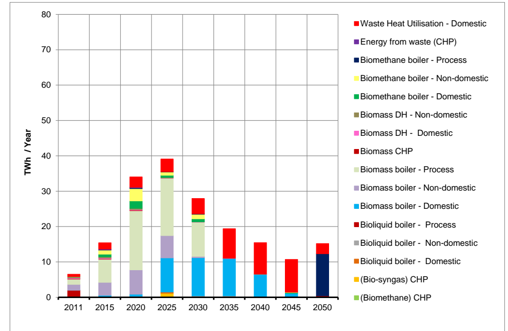
Figure 41 Bio-heat output (Core - lower resource scenario)
