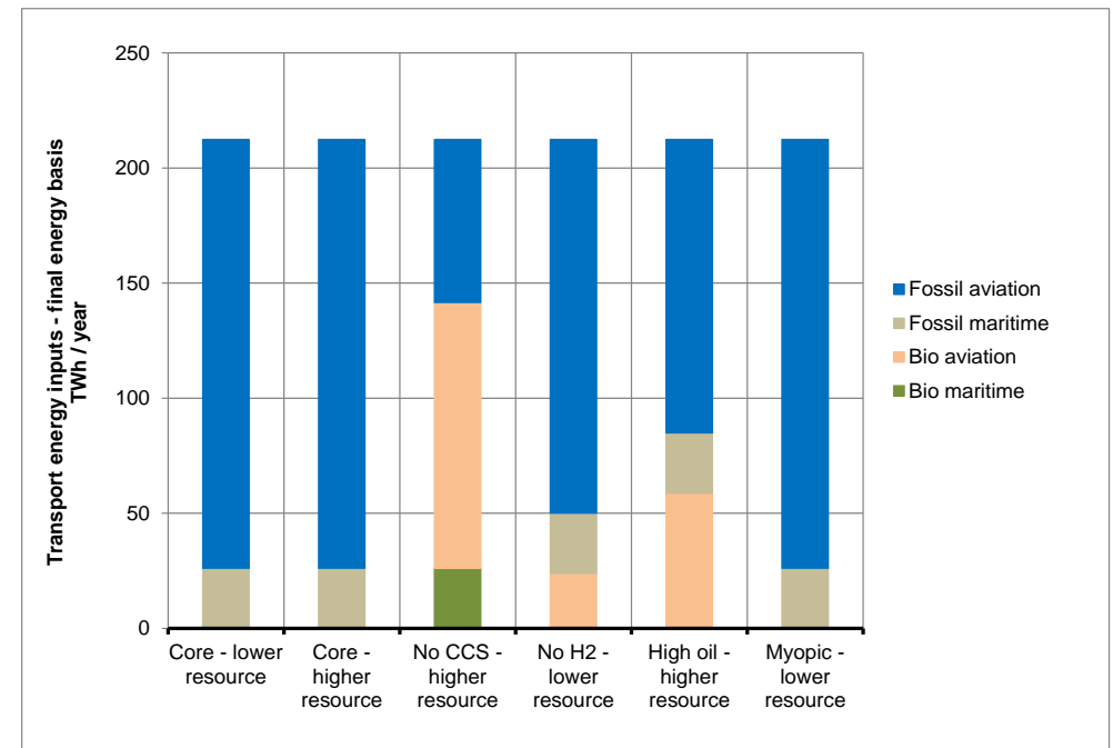
Figure 32 Non-road transport input (All scenarios 2050)
