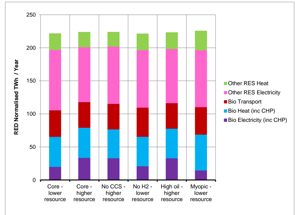
Figure 16 Normalised contribution to RED in 2020 (All scenarios)
