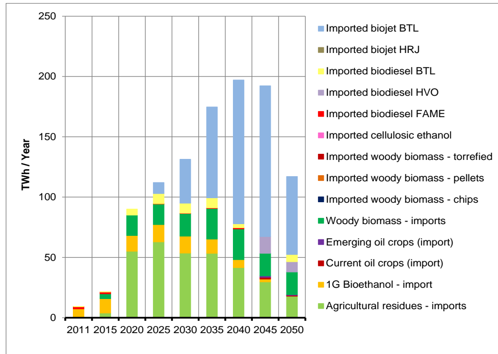
Figure 61 Bioenergy imports (No CCS - higher resource scenario)
