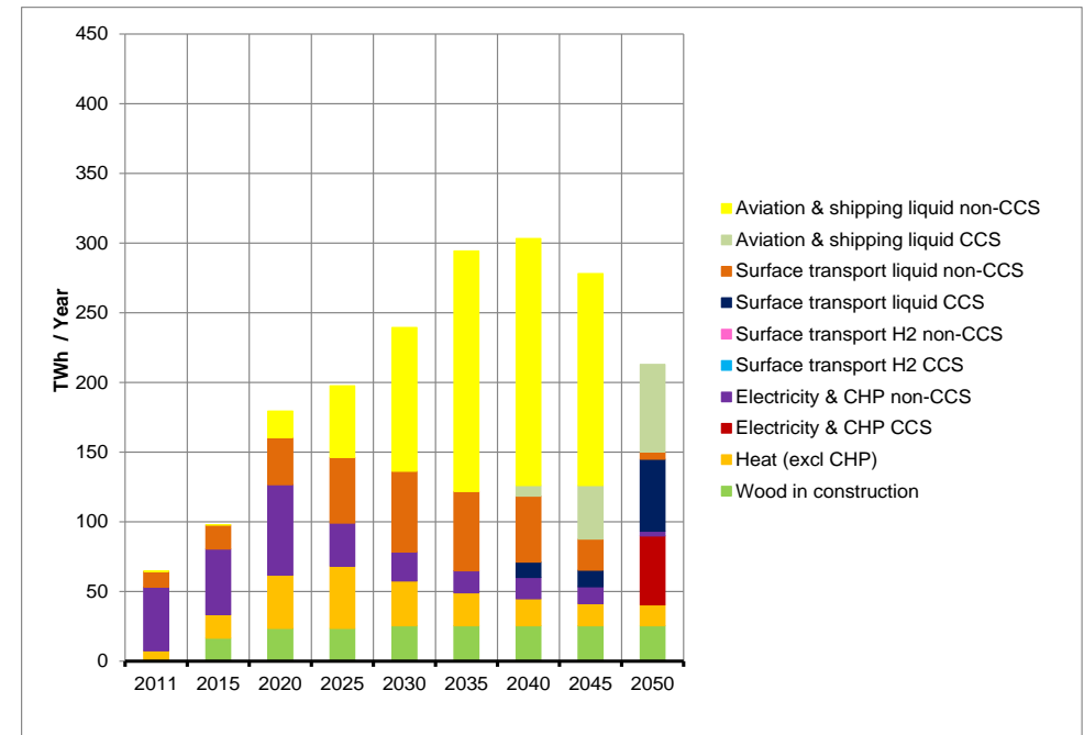
Figure 13 Primary bioenergy use (No H 2 - lower resource scenario)
