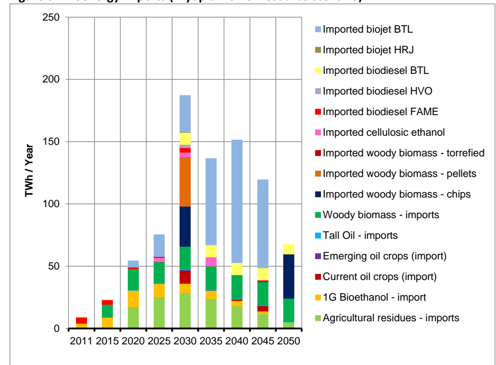
Figure 64 Bioenergy imports (Myopic - lower resource scenario)
