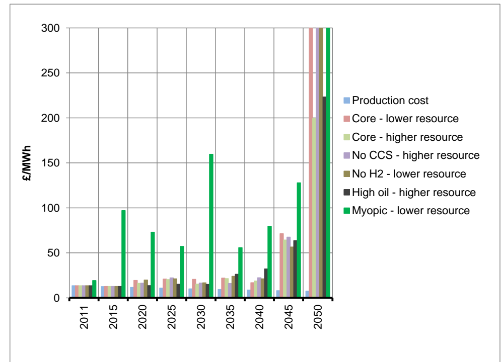
Figure 8 UK Energy crops shadow prices vs production costs (All scenarios)
