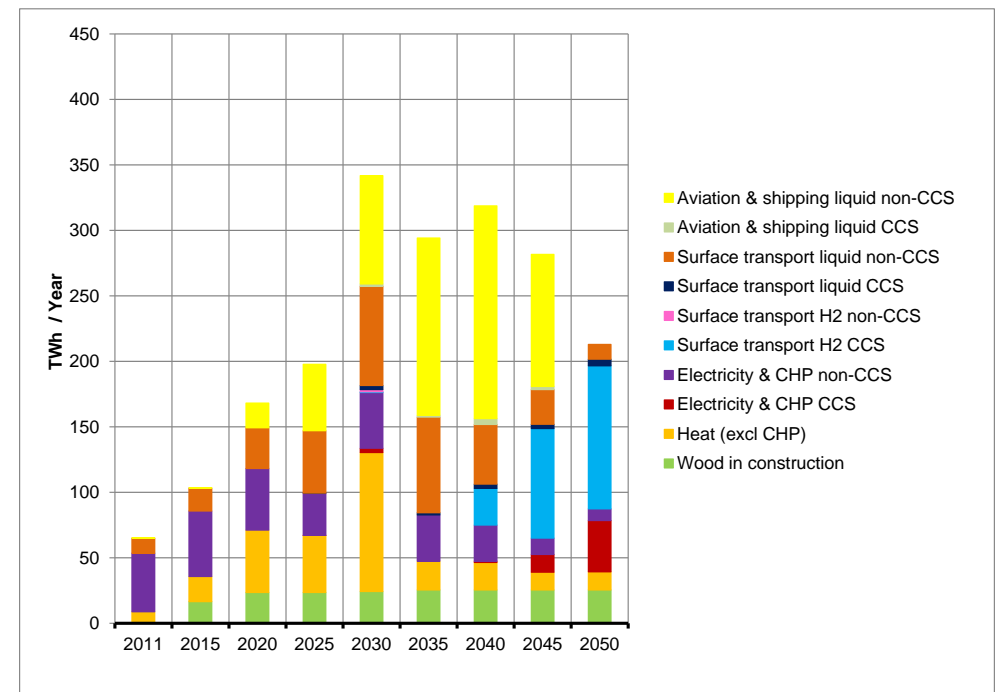
Figure 15 Primary bioenergy use (Myopic – lower resource scenario)
