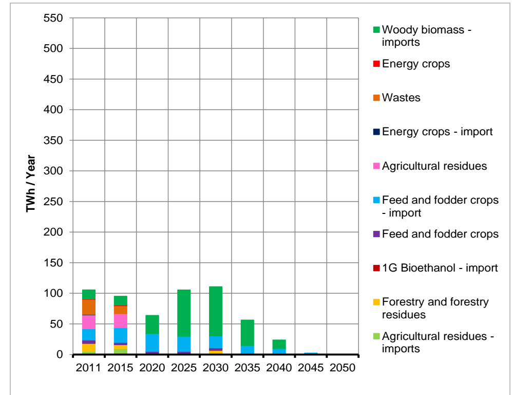
Figure 18 Bioresource unused (Core - lower resource scenario)
