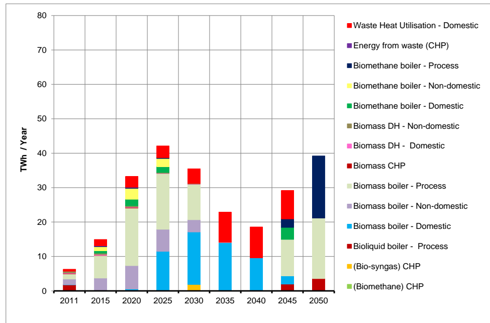
Figure 43 Bio-heat output (No CCS - higher resource scenario)
