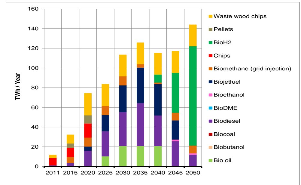
Figure 54 UK bioenergy carrier (Core - higher resource scenario)
