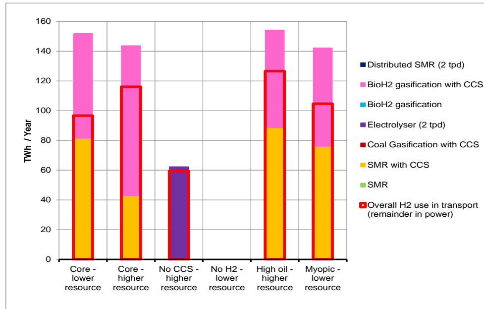
Figure 25 H 2 production (All scenarios 2050)
