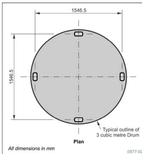
Figure 4 Layout of lifting features of 3 cubic metre drum
