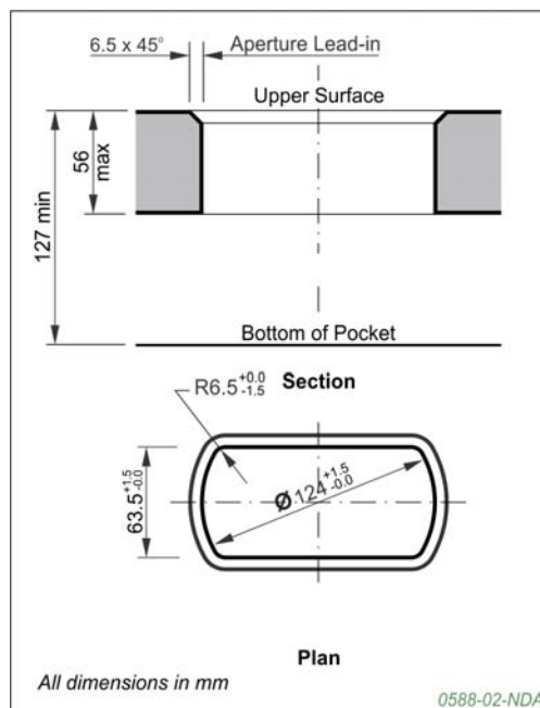
Figure 4 Layout of lifting features of 3 cubic metre drum
