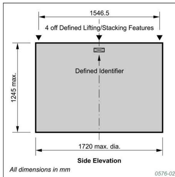
Figure 2 Standard features of the 3 cubic metre drum
