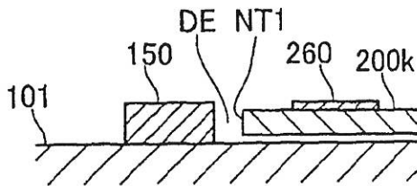
A-A CROSS SECTION
