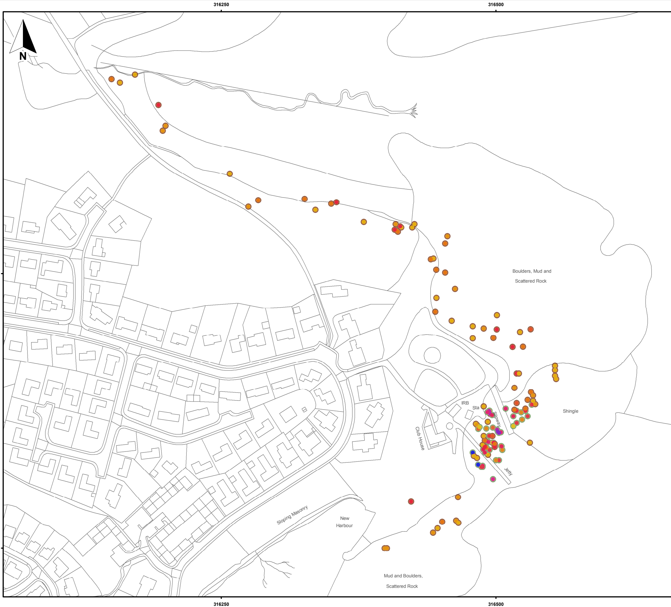
Figure 16: Spatial Distribution of Detected Point Sources
