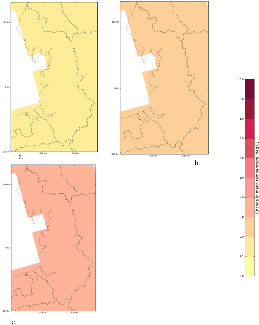
Figure H1 - Change in annual mean temperature (°C) in the 2050s under the Medium emissions scenario for the North West River Basin District for the a.) 10 per cent; b.) 50 per cent and c.) 90 per cent probability levels. Results from UKCP09.
