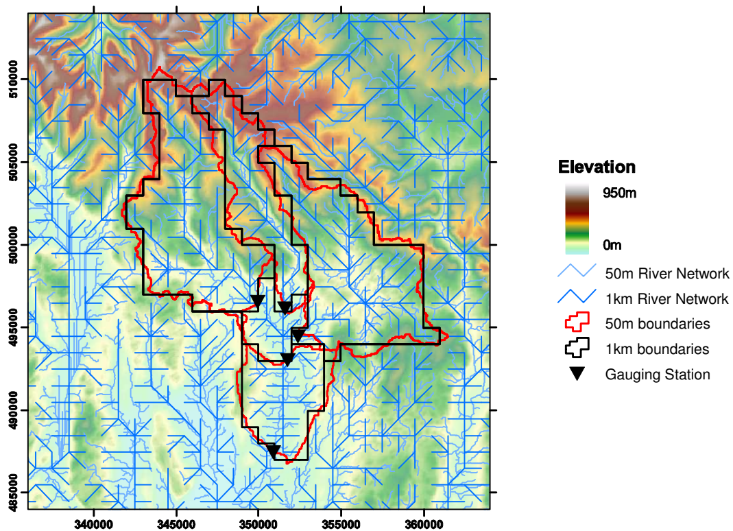
Figure 4.2 1km and IHD TM 50m resolution flow directions and catchment boundaries: River Kent catchment, Northwest England.
