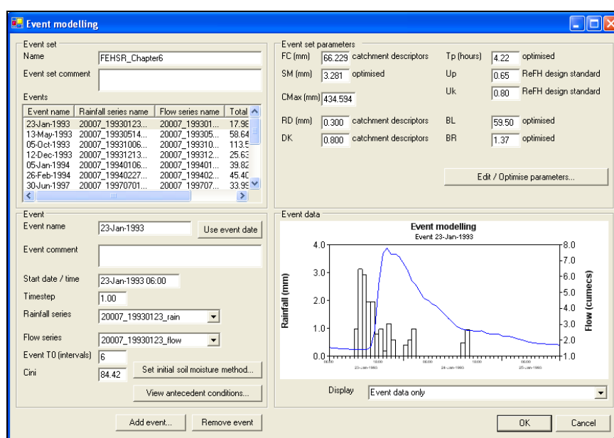
Figure 3.3 ReFH model parameter estimation start screen
