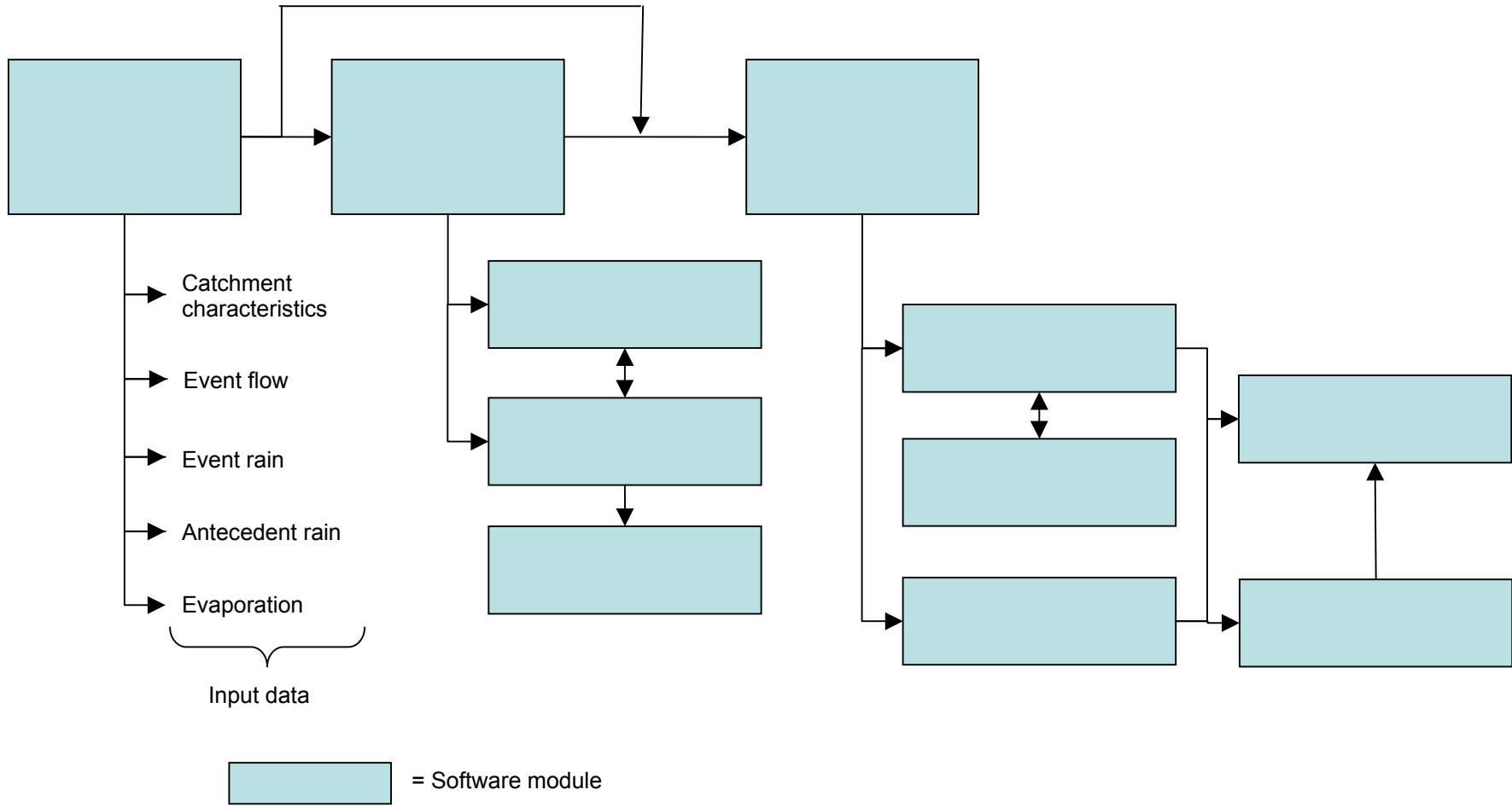
Figure 3.1 Schematic representation of the ReFH Flood Modelling software and the required input data
