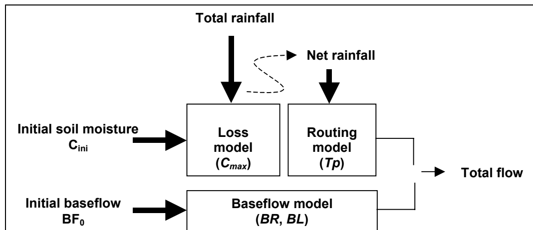
Figure 1.1 Schematic representation of the ReFH model
