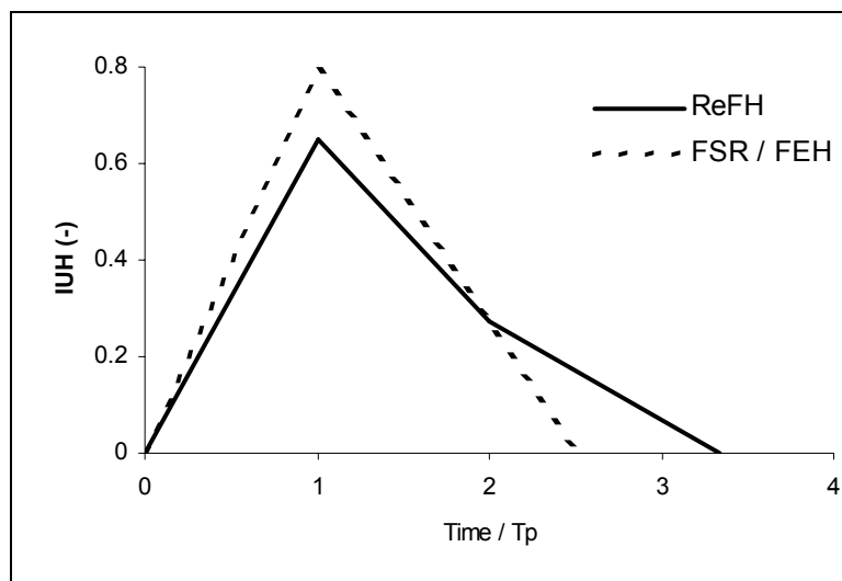
Figure 1.2 Comparison of the FSR/FEH and the ReFH standard shaped instantaneous unit hydrographs
