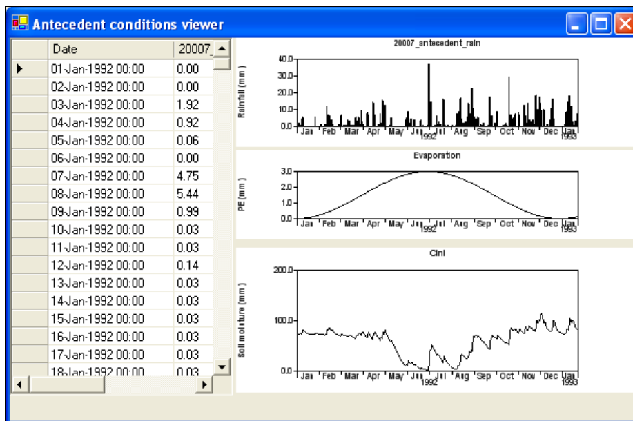
Figure 3.5 Daily average rainfall, evaporation and the resulting soil moisture content
