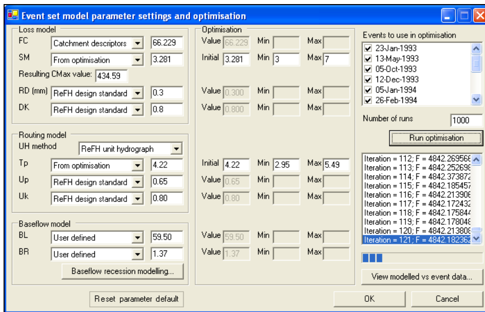
Figure 3.6 ReFH model parameter estimation functionality
