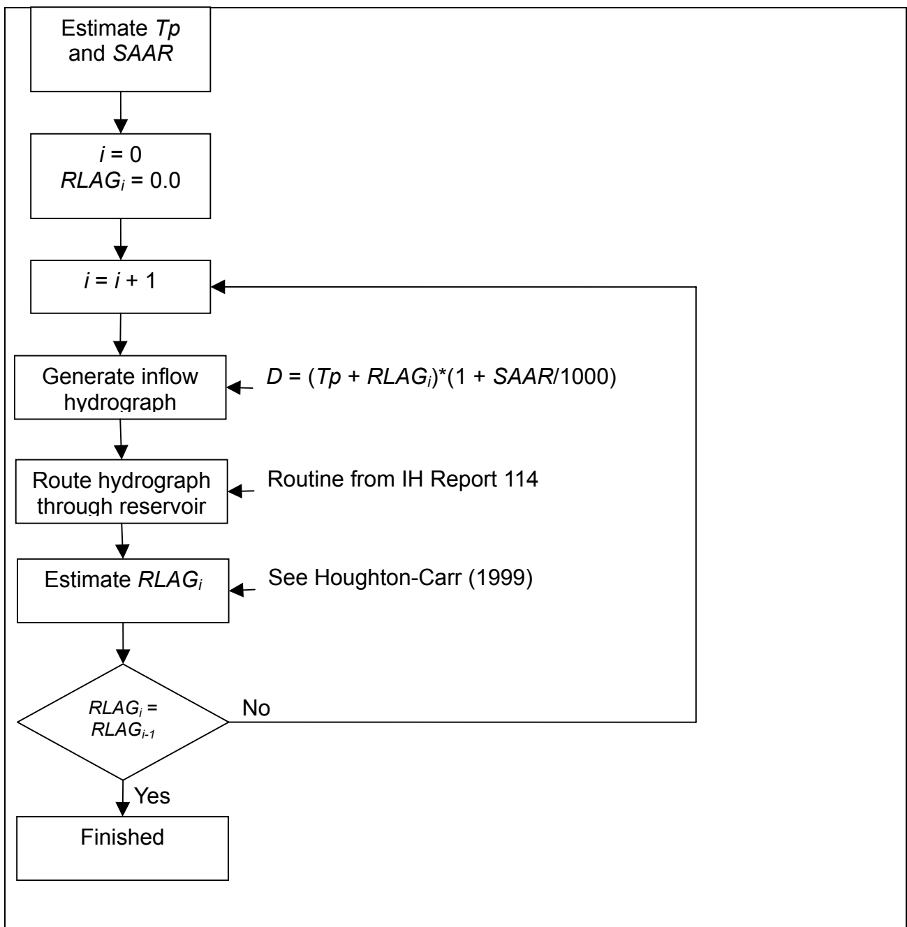
Figure 3.11 Procedure for estimation of reservoir lag RLAG
