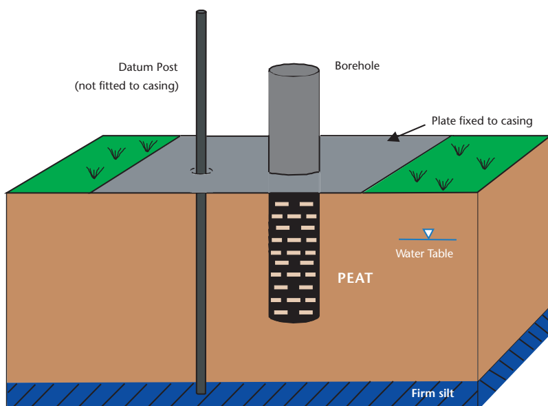
Figure 9 | Setting a borehole datum post
