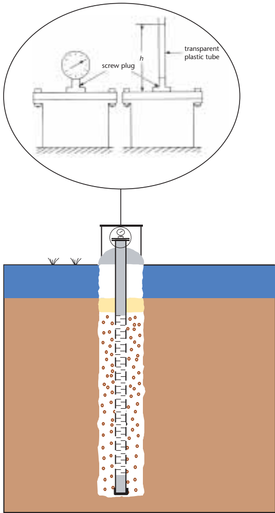
Figure 7 | Monitoring set-up for artesian conditions With permission from 'Field Hydrology' by Rick Brassington
