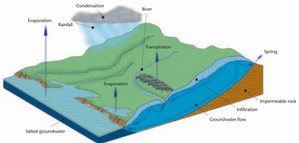
Figure 1 | The hydrological cycle With permission of the UK Groundwater Forum
