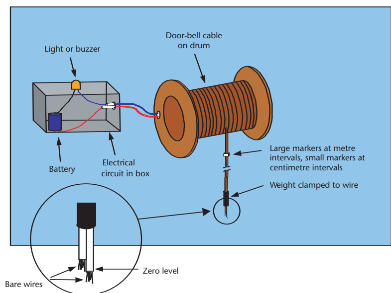
Figure 10 | Home-made dip-meter With permission from 'Field Hydrology' by Rick Brassington
