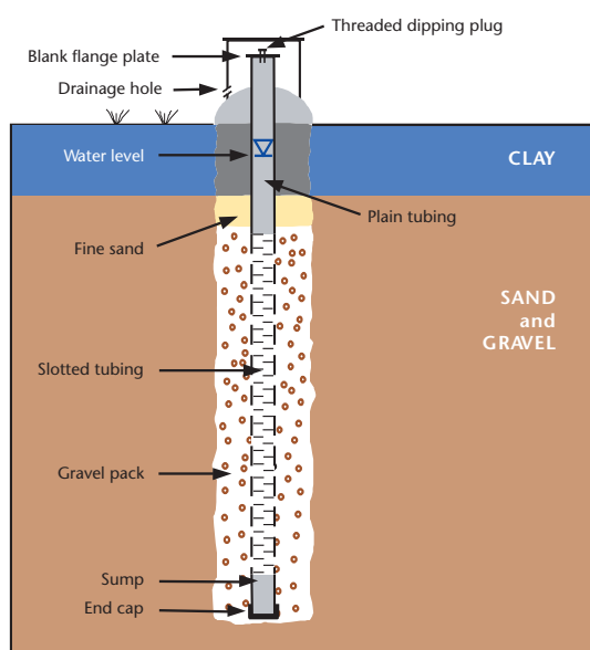
Figure 6 | Monitoring borehole for confined conditions
