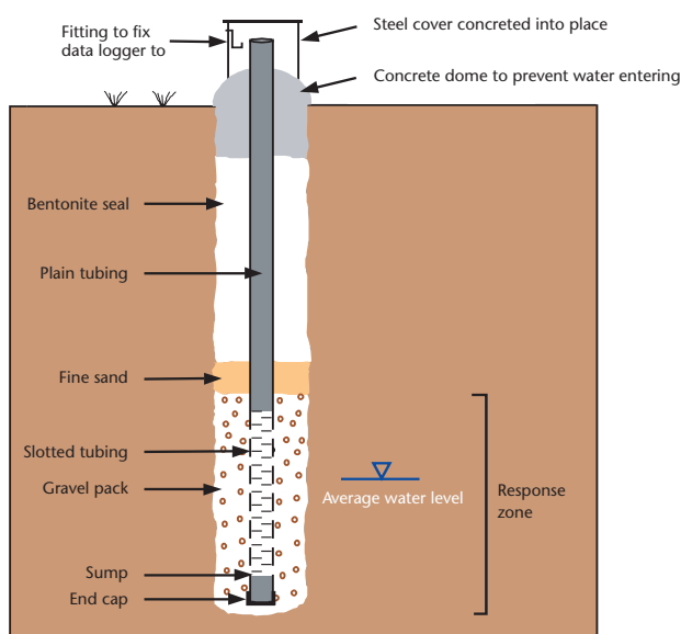
Figure 5 | Monitoring borehole
