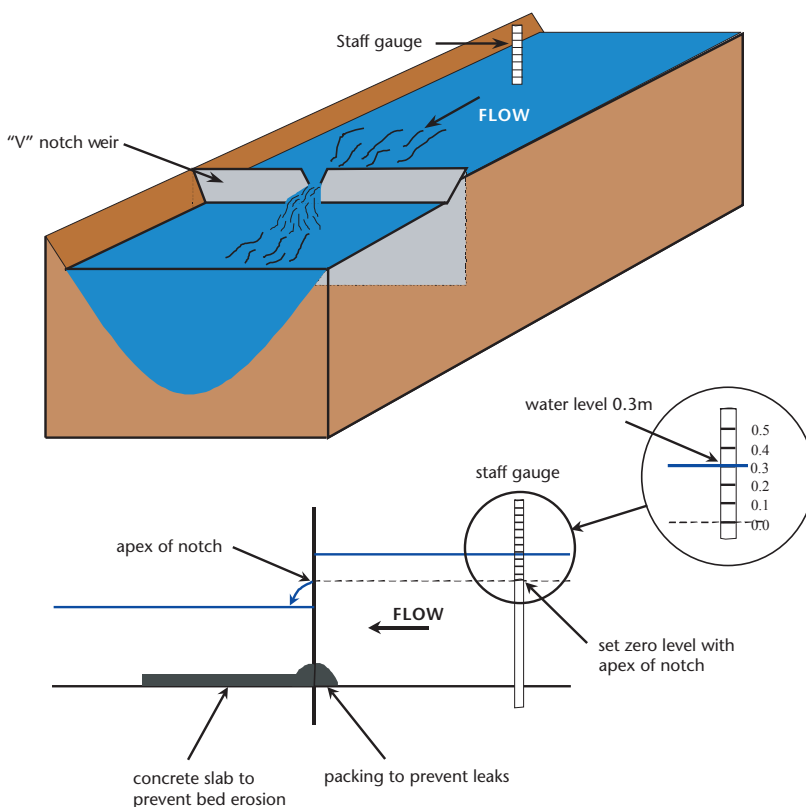
Figure 12 | 'V' notch weir With permission from 'Field Hydrology' by Rick Brassington
