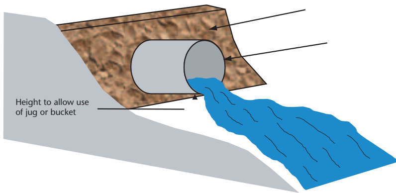
Figure 13 | Measuring spring flow using a catch-pit With permission from 'Field Hydrology' by Rick Brassington
