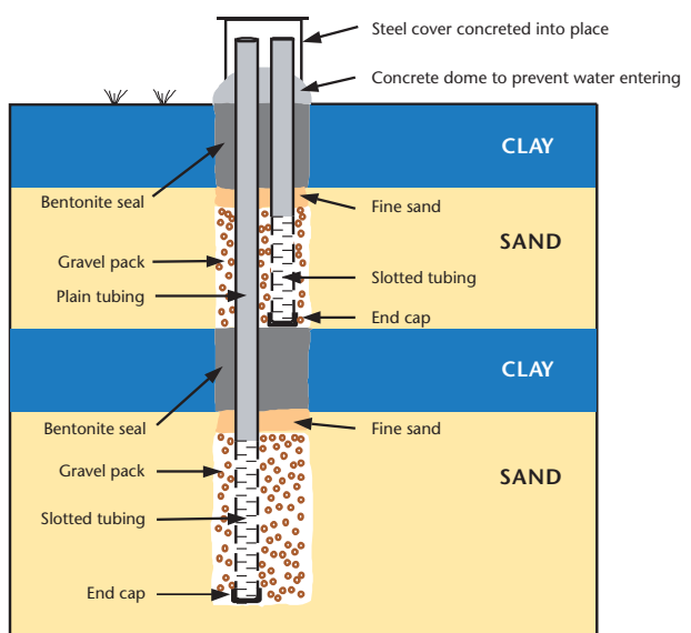
Figure 8 | Nested piezometer
