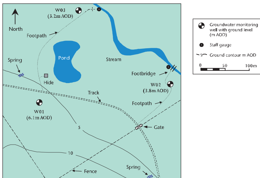
Figure 4 | Base plan
