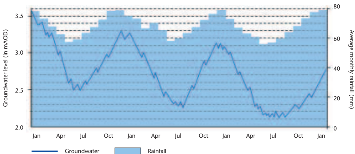
Figure 14 | Example hydrograph
