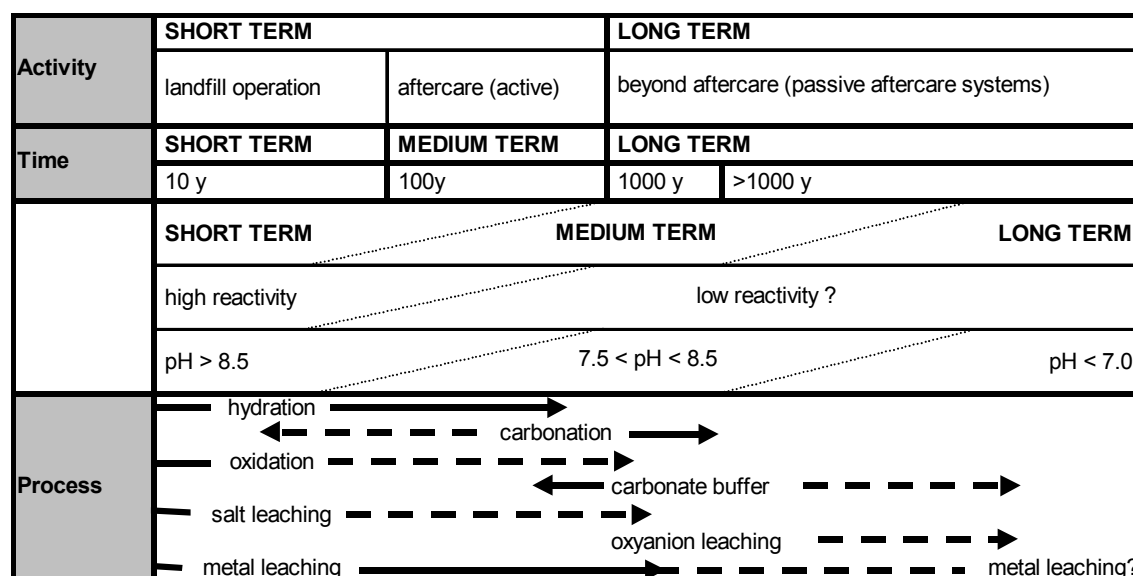
Figure 14 Classification of time scales relevant to landfilling (after Sabbas et al. , 2003)
