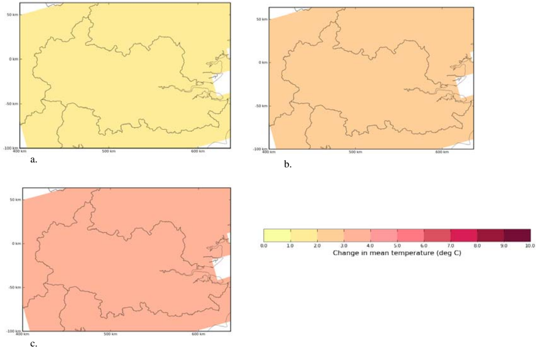
Figure H.1 Change in annual mean temperature (°C) in the 2050s under the Medium emissions scenario for the Thames River Basin District for the a.) 10 per cent; b.) 50 per cent and c.) 90 per cent probability levels. Results from UKCP09.
