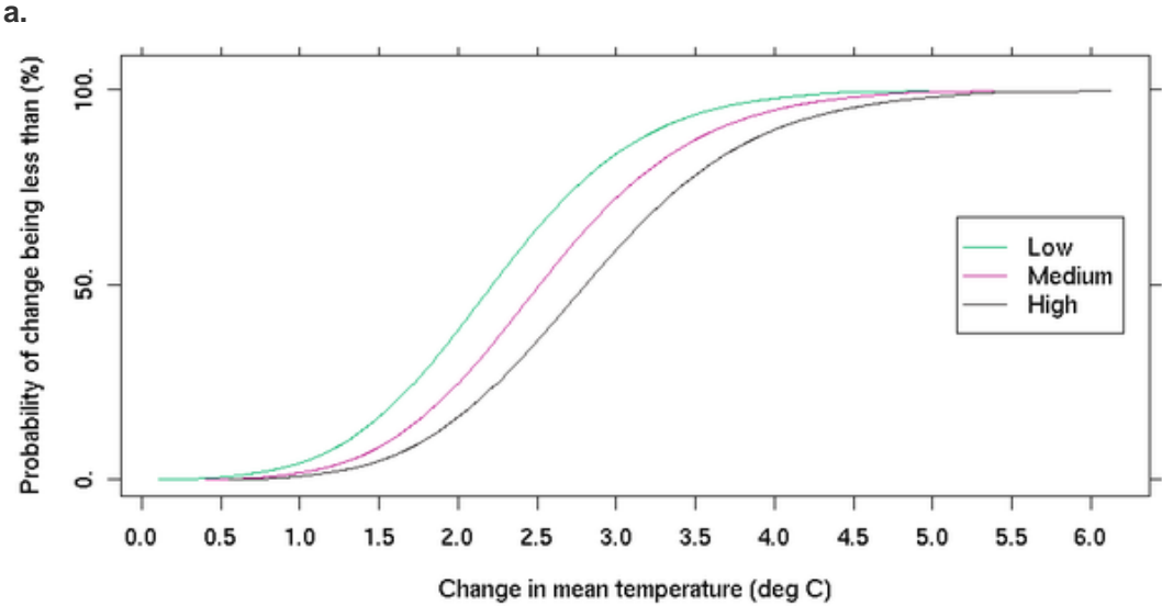
Figure H.4 Change in a.) annual mean temperature (°C), b.) summer precipitation (per cent) and c.) winter precipitation (per cent) in the 2050s for the Thames River Basin District plotted as cumulative distribution functions for the low, medium and high emissions scenarios. Results from UKCP09.
