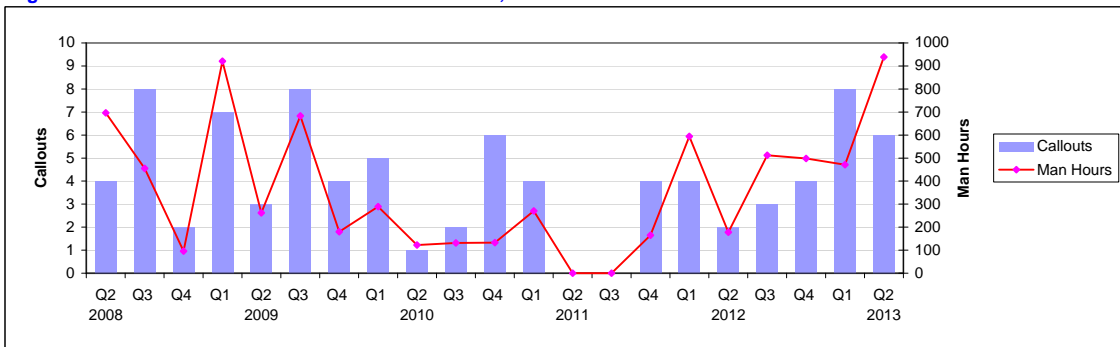
Figure 13d Callouts and Man Hours for MRT Valley, 2008 Q2 to 2013 Q2
